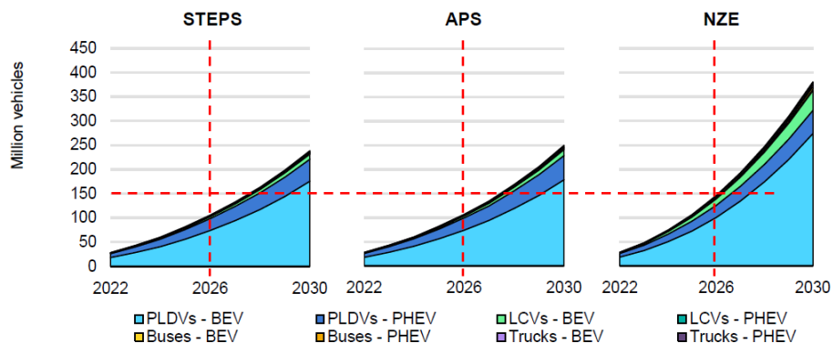
Electric vehicle stock by mode and scenario, 2022-2030
